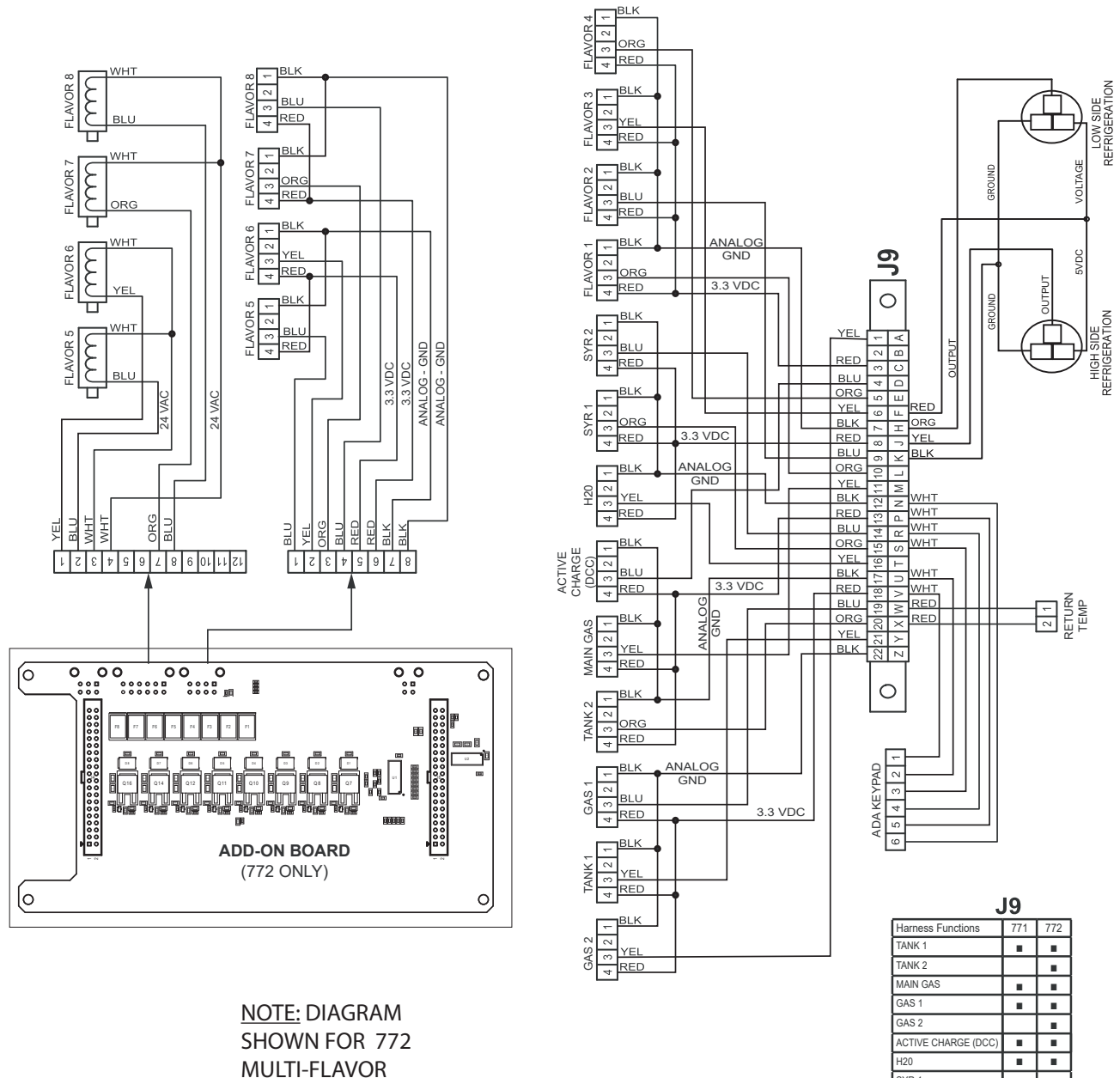
Figure 11.4 Electrical Diagram for 771 and 772 Multi-Flavor Dispensers (1 OF 3)
