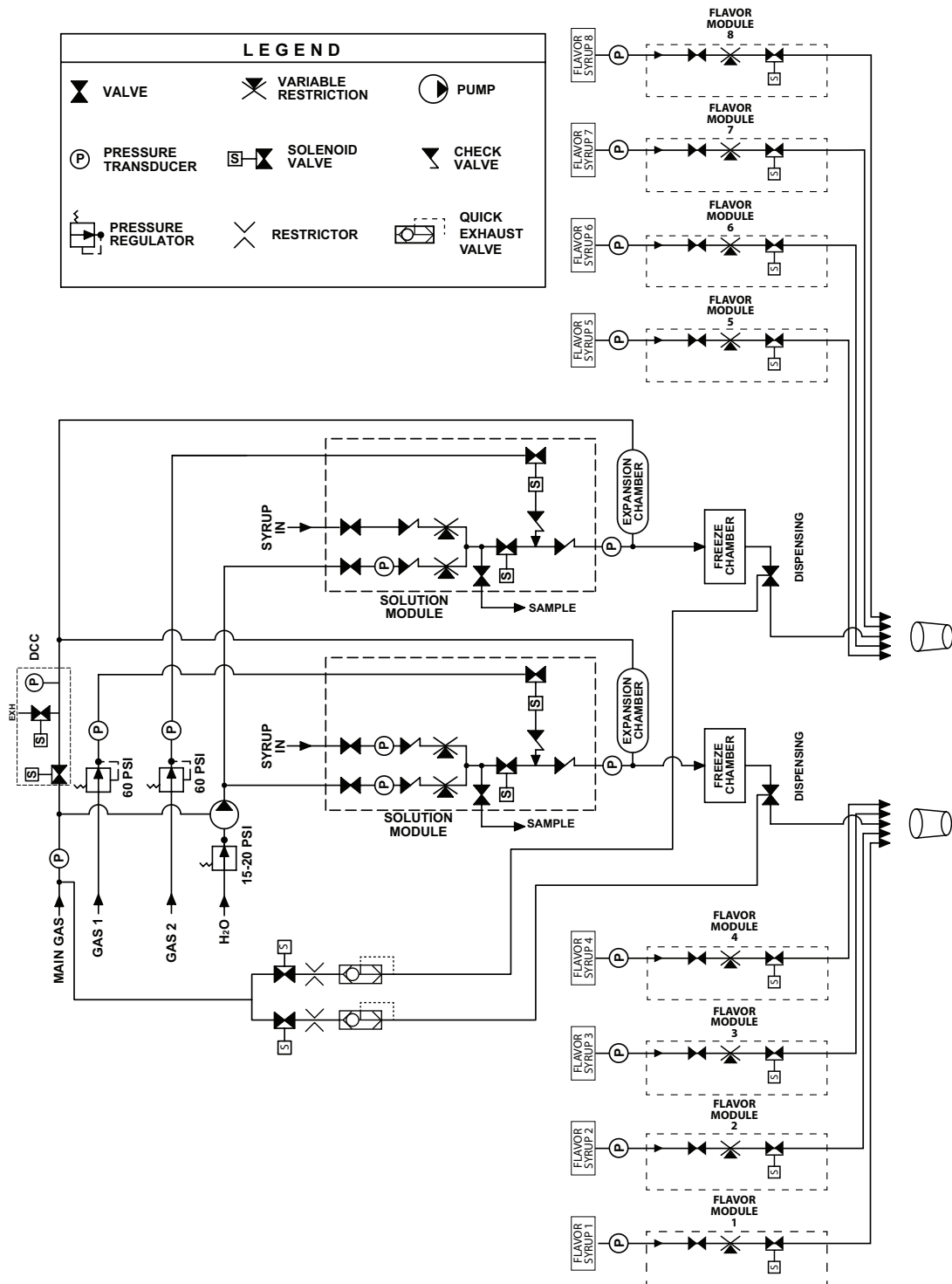
Figure 11.2 Flow Diagram for 772 Multi-Flavor Dispenser
