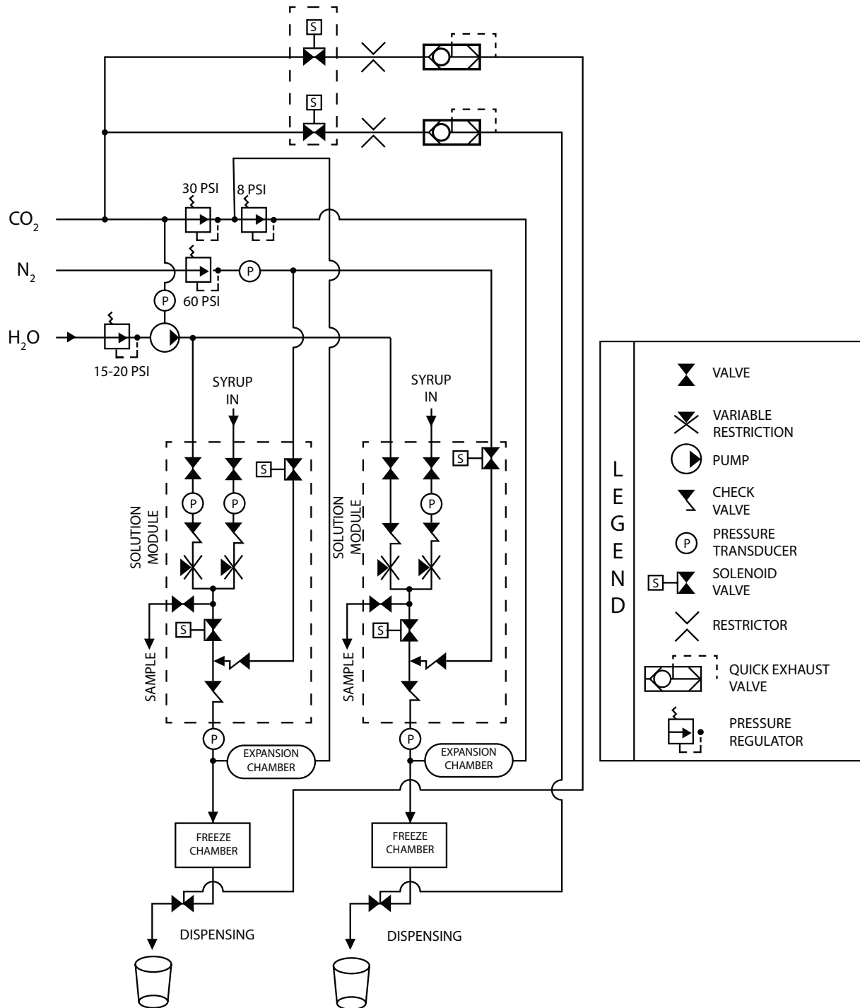
Figure 11.5 Flow Diagram for 372 Nitro Dispenser
