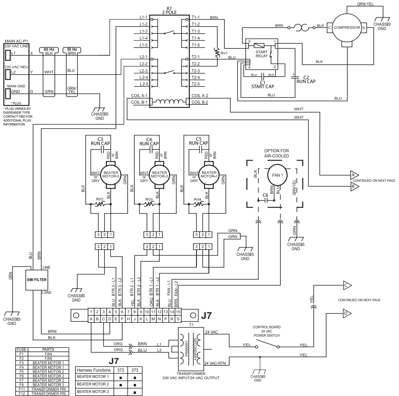
Figure 11.7 Electrical Diagram for 372 Standard Dispenser 1 OF 3
