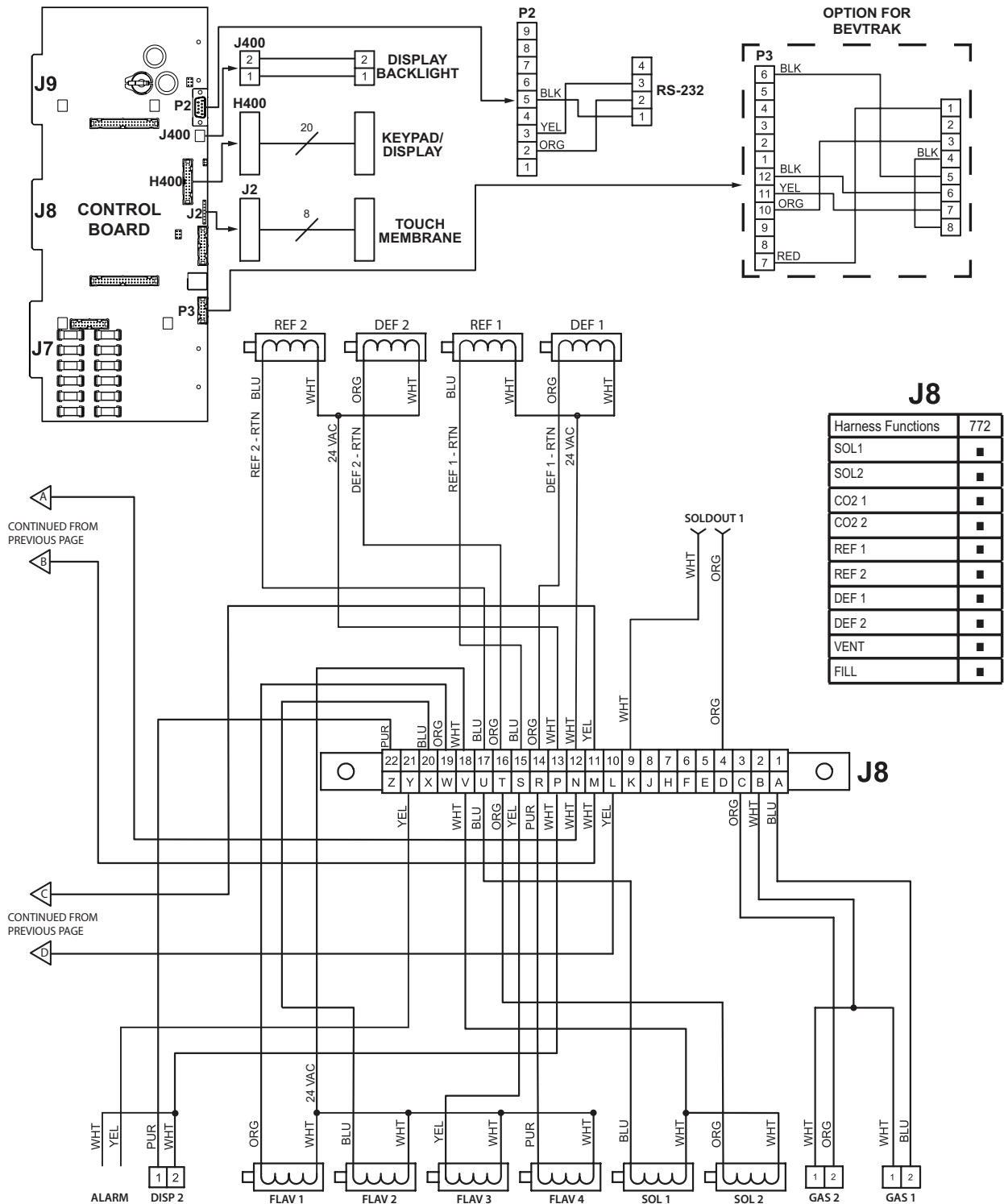
Figure 11.11 Electrical Diagram for 372 Multi-Flavor Dispenser 2 OF 3
