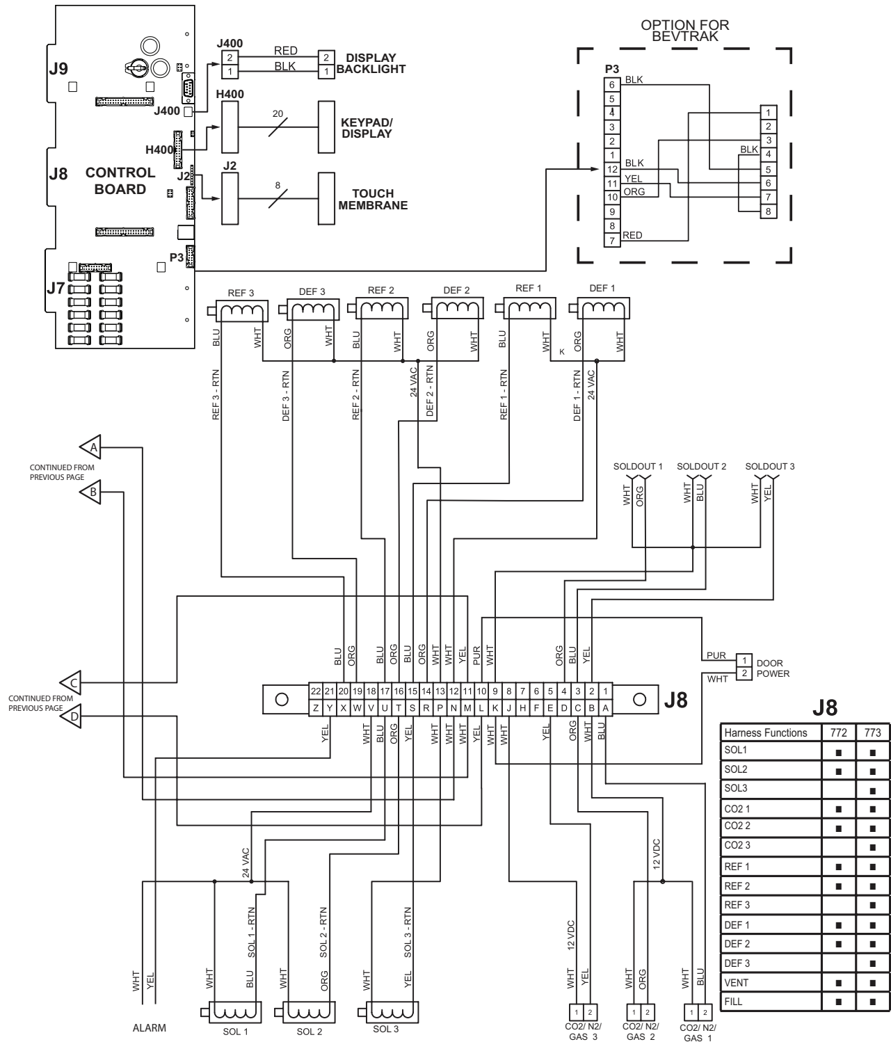
Figure 11.8 Electrical Diagram for 372 Standard Dispenser 2 OF 3
