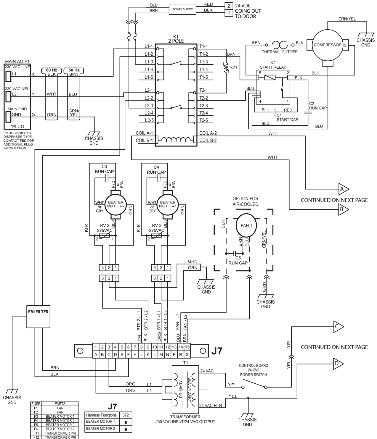
Figure 11.10 Electrical Diagram for 372 Multi-Flavor Dispenser 1 OF 3
